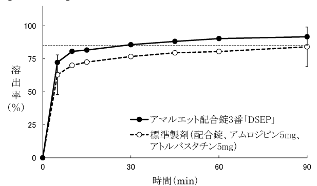
pH5.0/50rpm
