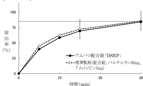
pH3.0/50rpm
