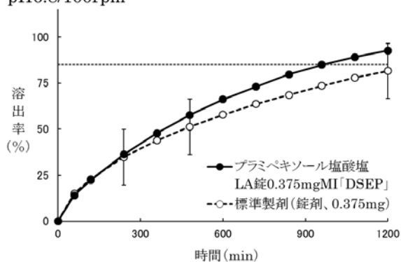
pH6.8/100rpm
