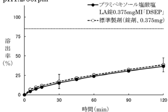
pH1.2/50rpm
