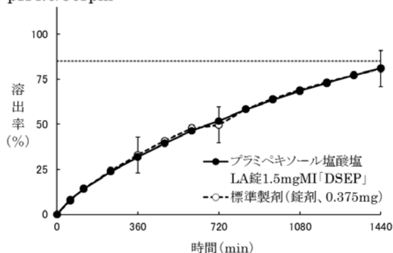
pH4.0/50rpm
