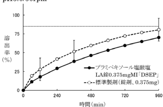
pH3.0/50rpm
