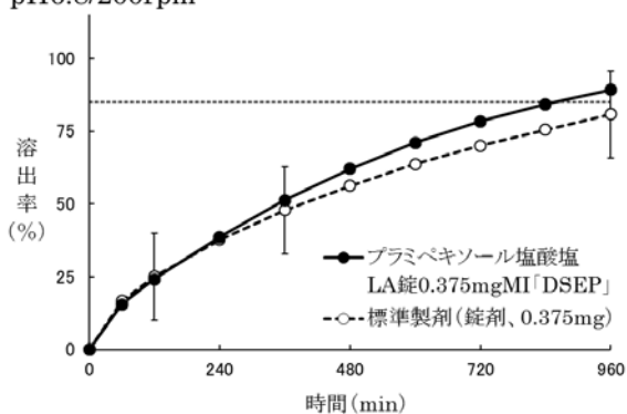
pH6.8/200rpm
