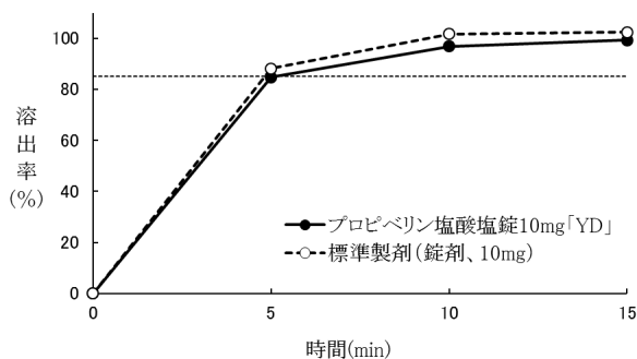
pH6.8/50rpm
