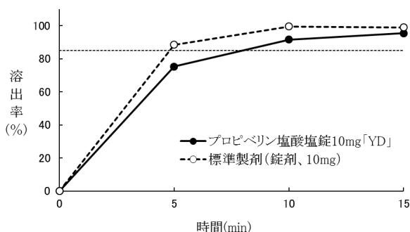
pH6.8/50rpm
