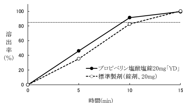
pH3.0/50rpm
